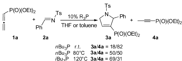
Scheme 2. [3+2] Annulation of diethyl allenylphosphonate ( 1a ) with N -tosylbenzalimine ( 2a ).
