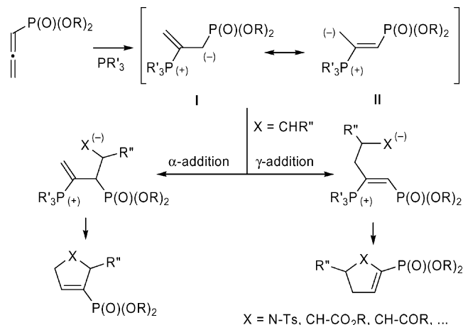
Scheme 1. Activation of allenylphosphonates by nucleophilic phosphanes.
